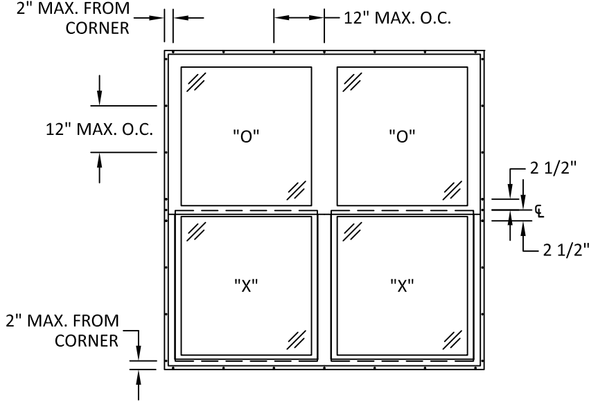
ANCHOR LAYOUT 72" X 72", TWIN UNIT
