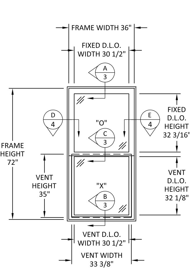
TYPICAL ELEVATION NO KEEPER
