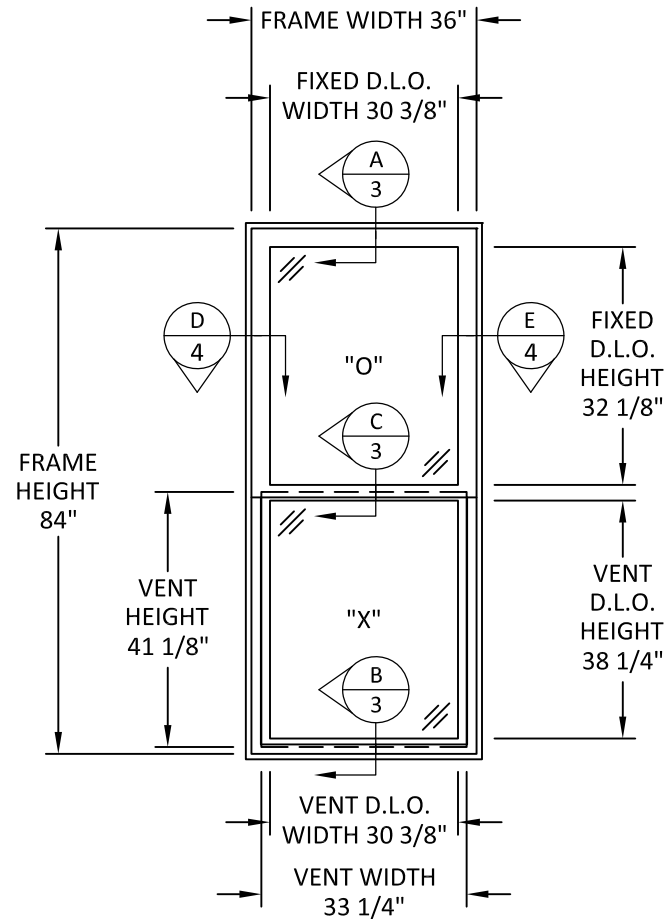
TYPICAL ELEVATION
