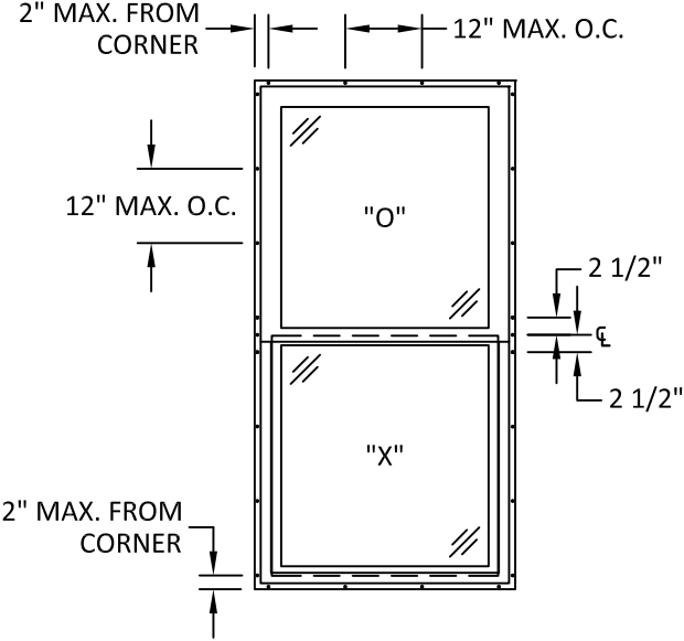
ANCHOR LAYOUT 36" X 72" UNIT
