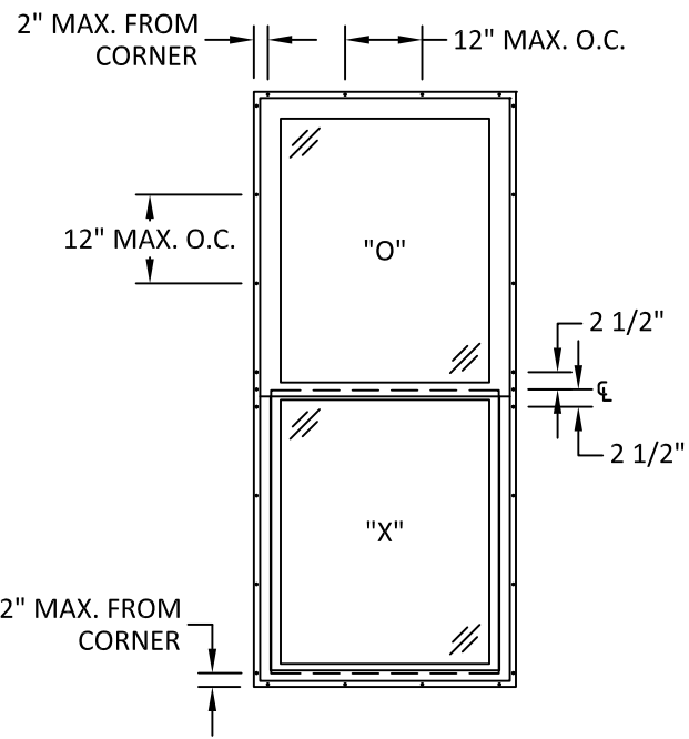
ANCHOR LAYOUT 36" X 84" UNIT
