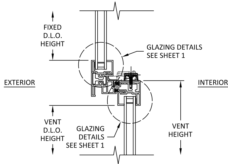
C 3 VERTICAL SECTION MEETING RAIL
