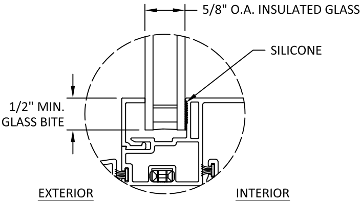
GLAZING DETAIL VENT LITE
